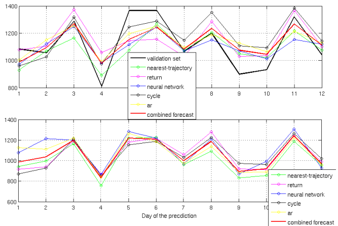
Fig. 2. The figure on top shows the outcome of the individual models (nearest trajectory model, difference/return model, feed-forward neural network model, trend cycle model and auto regressive (AR) model) for the left-out part of the time series (number 42 in the challenge). The SMAPE of these models defines the weight for the combined forecast. The final outcome of this approach that entered the CIF challenge is shown on the bottom (solid red line).
